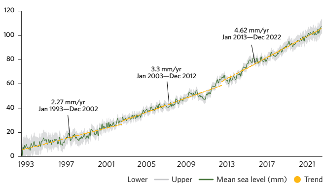
Global mean sea level, 1993–2022 (millimetres)
